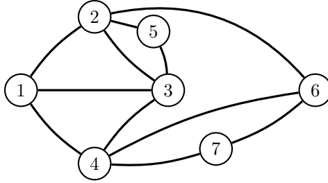
FIGURE 2. This graph represents the block B = (1) \uplus (2, 3, 1) \uplus (4, 3) \uplus (5, 2) \uplus (6, 4) \uplus (7, 6) . The path decomposition of Substep 2.3 can be chosen in this case as \mathfrak{L}^1 = (1, 2, 6) , \mathfrak{L}^2 = (1, 4, 7, 6) , and \mathfrak{L}^3 = (1, 3, 2, 5, 3, 4, 6) .
