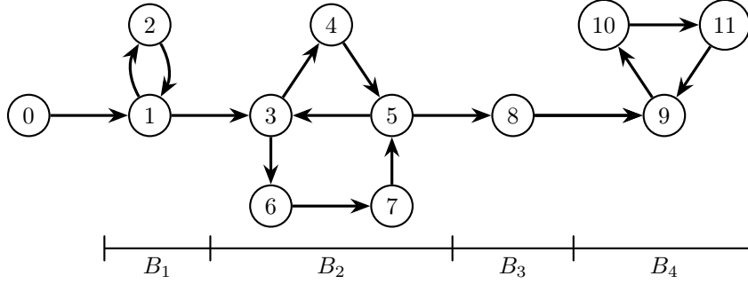
FIGURE 1. Each term in (4.57) can be represented by means of a directed graph on the index set \{0\} \cup [k] , where edges are given by pairs of consecutive elements in B_1 \uplus \dots \uplus B_r with possible multiplicities and where we include the edge (0, b) with b the root of B_1 . In this way, an edge to i corresponds to an operator \mathcal{J}_{L; x_T}^{x_i} in (4.57). For instance, the above diagram is associated to blocks B_1 = (1) \uplus (2, 1) , B_2 = (3) \uplus (4, 5, 3) \uplus (6, 7, 5) , B_3 = (8) , and B_4 = (9) \uplus (10, 11, 9) .
